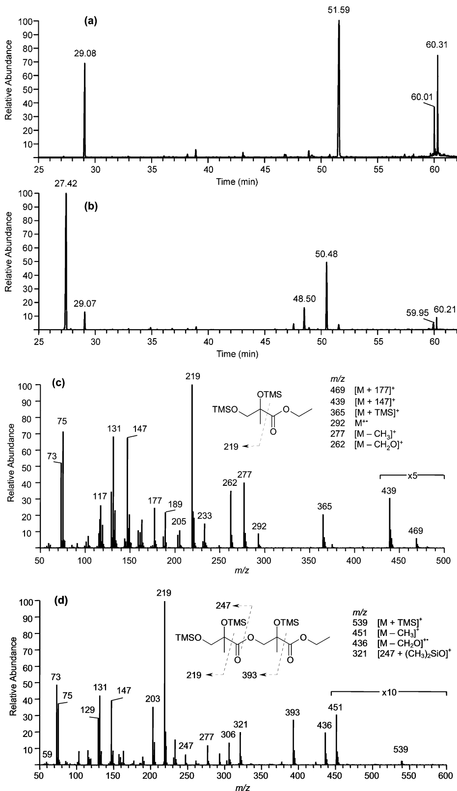
Figure 15. (a) GC/MS EIC ( = m/z 219) for high-NO x isoprene nucleation sample (Experiment 5) treated only with TMS derivatization. (b) GC/MS EIC ( = m/z 219) for a duplicate sample of the same experiment (Experiment 5) in part a, but treated this time by hydrolysis/ethylation followed by TMS derivatization. (c) EI mass spectrum for ethyl ester of 2-MG acid detected in part b ( RT = 27.42 min). (d) EI mass spectrum for ethyl ester of linear 2-MG acid dimer detected in part b ( RT = 50.48 min). The hydrolysis/ethylation followed by TMS derivatization results presented here confirm the existence of polyesters in high-NO x SOA.
